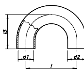
CURVA 180° SOLDAR LARGA LONG WELD.BEND 180° COUDE 180° LONG. A SOUDER
